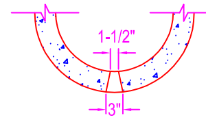
DRAIN HOLE DETAIL
